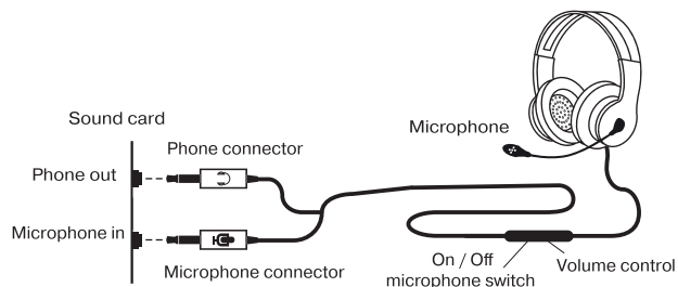
Fig. 1. Connection diagram
